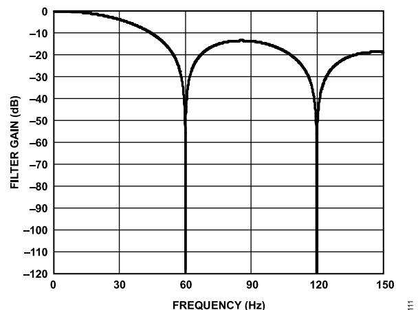
Figure 102. 60 Hz Rejection
