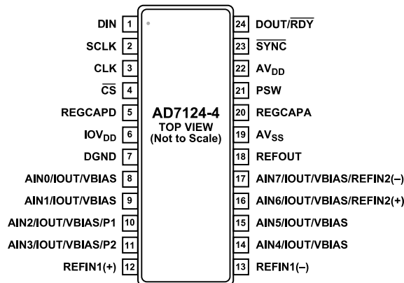
Figure 10. 24-Lead TSSOP Pin Configuration
