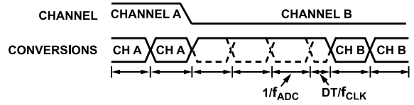
Figure 91. Sinc 3 Channel Change
