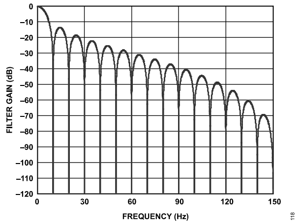
Figure 109. Simultaneous 50 Hz and 60 Hz Rejection
