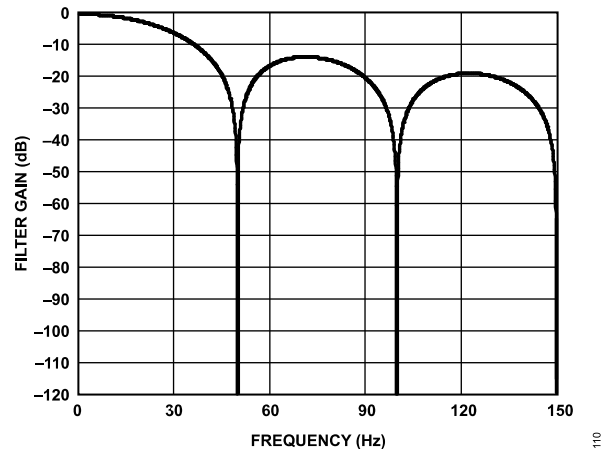
Figure 101. 50 Hz Rejection
