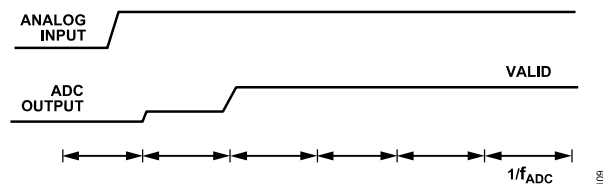
Figure 100. Step Change on the Analog Input, \text{Sinc}^4 + \text{Sinc}^1 Filter
