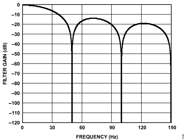
Figure 107. 50 Hz Rejection
