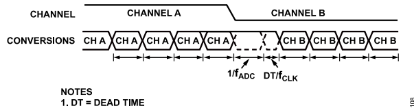
Figure 99. Fast Settling, \text{Sinc}^4 + \text{Sinc}^1 Filter
