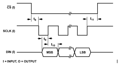
Figure 5. Write Cycle Timing Diagram
